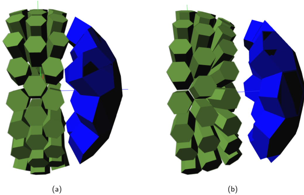
Figure 18: The proposed geometries of the coupling of NEDA (green, left-hand-side) and the Neutron Wall (blue, right-hand-side) for the AGATA campaign at GANIL.
