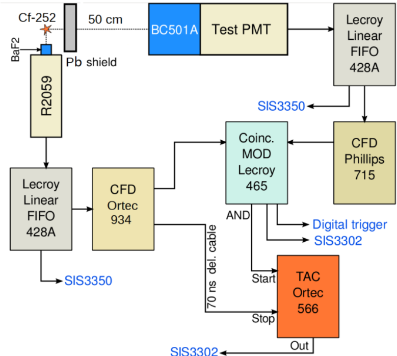
Figure 59: Block scheme of the experimental arrangement.
