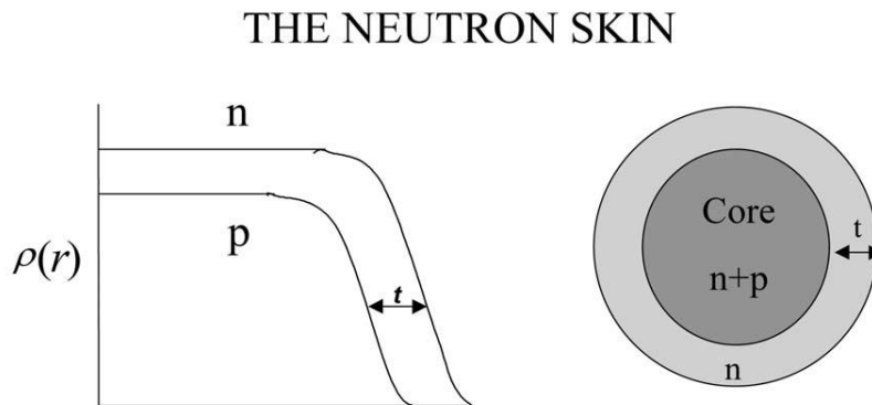
Figure 1: Schematic illustration of the neutron skin. For more extended neutron distributions one expects a reduction of the spin-orbit term of the residual nucleon-nucleon interaction [7].
