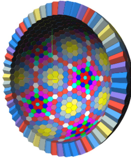
Figure 17: This spherical configuration was designed as a realistic reference. It consists of 606 detector units with 16 different shapes, covers a solid angle of almost 2\pi sr at a distance of 1 m from the target position.
