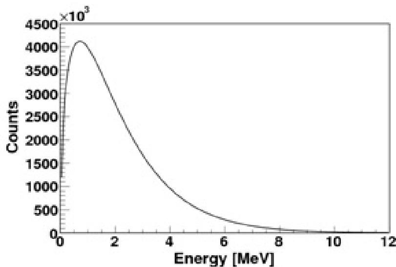
Figure 14: Energy distribution of ^{252}\text{Cf} neutrons according to eq. (1).
