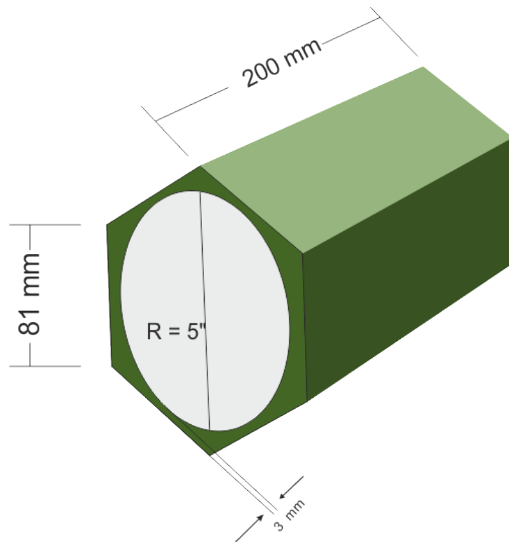
Figure 15: Schematic picture of the NEDA detector unit.
