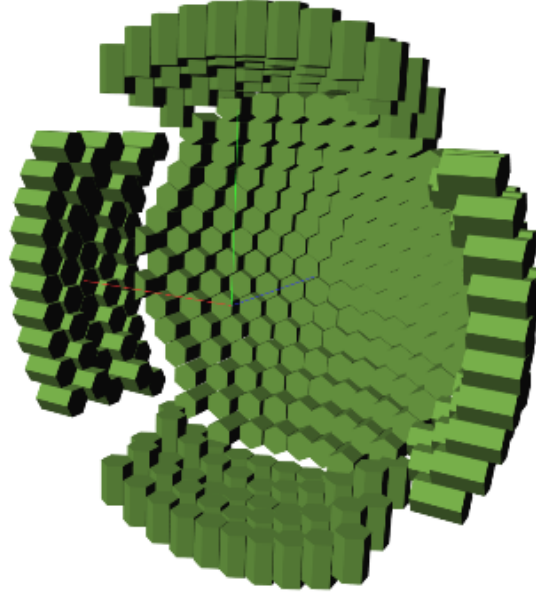
Figure 16: The proposed geometry of NEDA 2\pi consisting of 355 detector units and covering a solid angle of 1.88\pi sr at a distance of 1 m from the target position.
