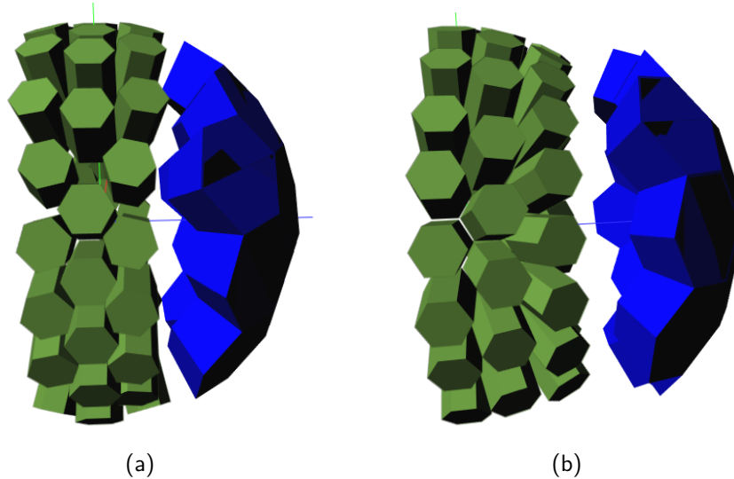
Figure 18: The proposed geometries of the coupling of a) 46 and b) 50 NEDA detectors (green, left-hand-side) and 50 Neutron Wall detectors (blue, right-hand-side) for the AGATA campaign at GANIL.
