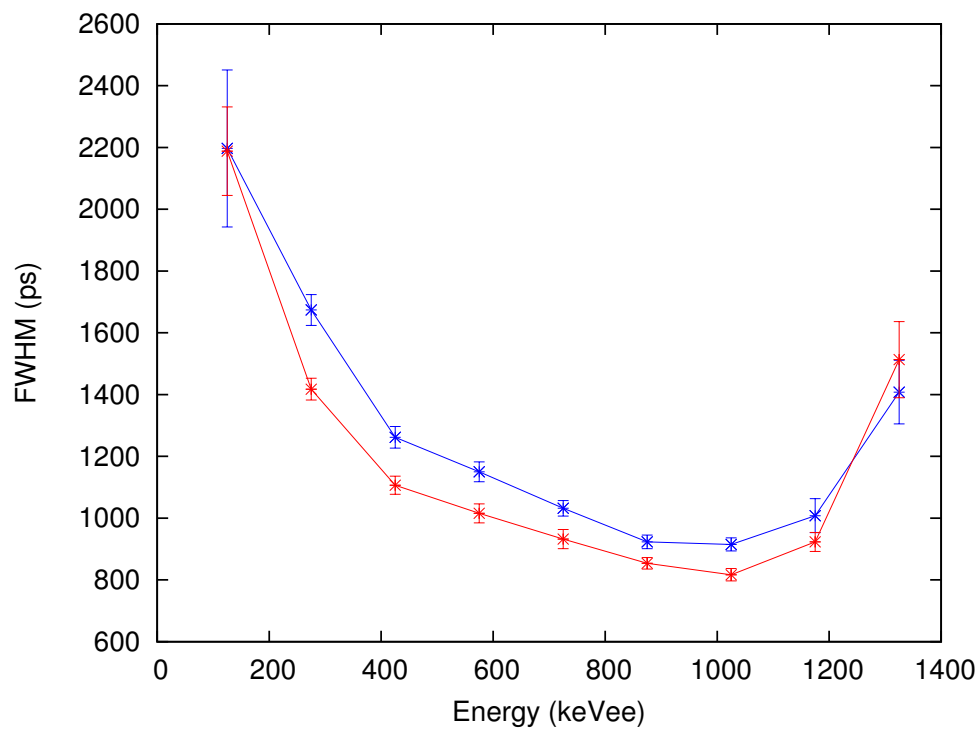
Figure 73: Time resolution (FWHM) versus signal amplitude measured with a ^{60}\text{Co} source, the NEDA prototype detector and a \text{BaF}_2 detector. The width of the energy window was 100 keV. Blue: digital measurements. Red: analogue measurements. The results are preliminary.
