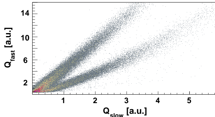
Figure 74: Neutron- \gamma discrimination of the NEDA prototype detector using the charge-comparison method. See text for the definition of Q_{\text{fast}} and Q_{\text{slow}} . The results are preliminary. JN: this figures is mostly empty. can you make a better one?
