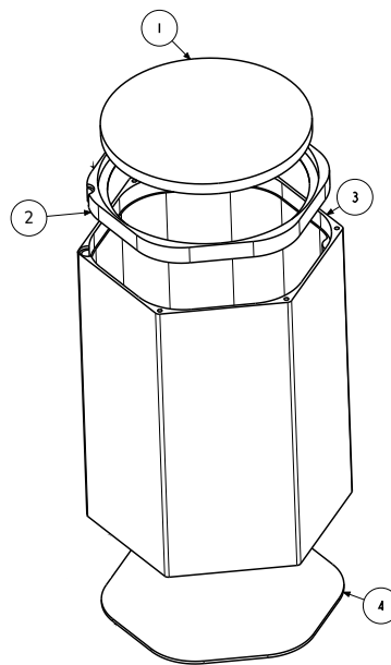
Figure 71: Cell construction process by welding two flanges to the hexagonal cylinder. 1) Glass window . 2) Top flange. 3) Cylinder. 4) Bottom lid.
