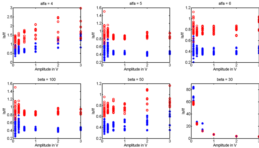
Figure 46: \hat{l}_S/\hat{l}_F versus signal amplitude. Upper: sweep across several \alpha values with \beta = 100 . Lower: sweep across several \beta values with \alpha = 5 . Events produced by \gamma rays are plotted as blue stars and neutrons as red circles.
