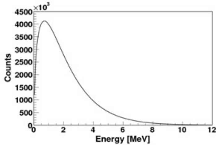
Figure 14: Energy distribution of ^{252}\text{Cf} neutrons according to eq. (1) with T = 1.42 \text{ MeV} . JN: Grzes promised to send a figure with better image quality.
